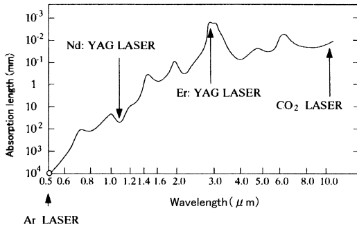
Fig. 1 Absorption spectrum of water 7)
